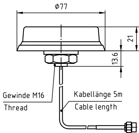
Antenna GSM 5m Teile-Nr./Part No. P8000007506
