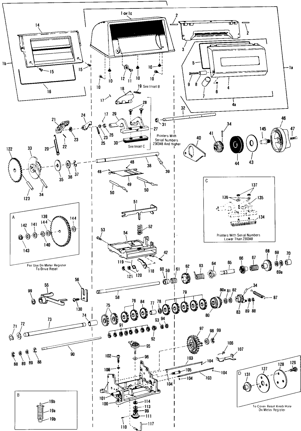
Meter Duplicator Zero Start (Reset) Type
