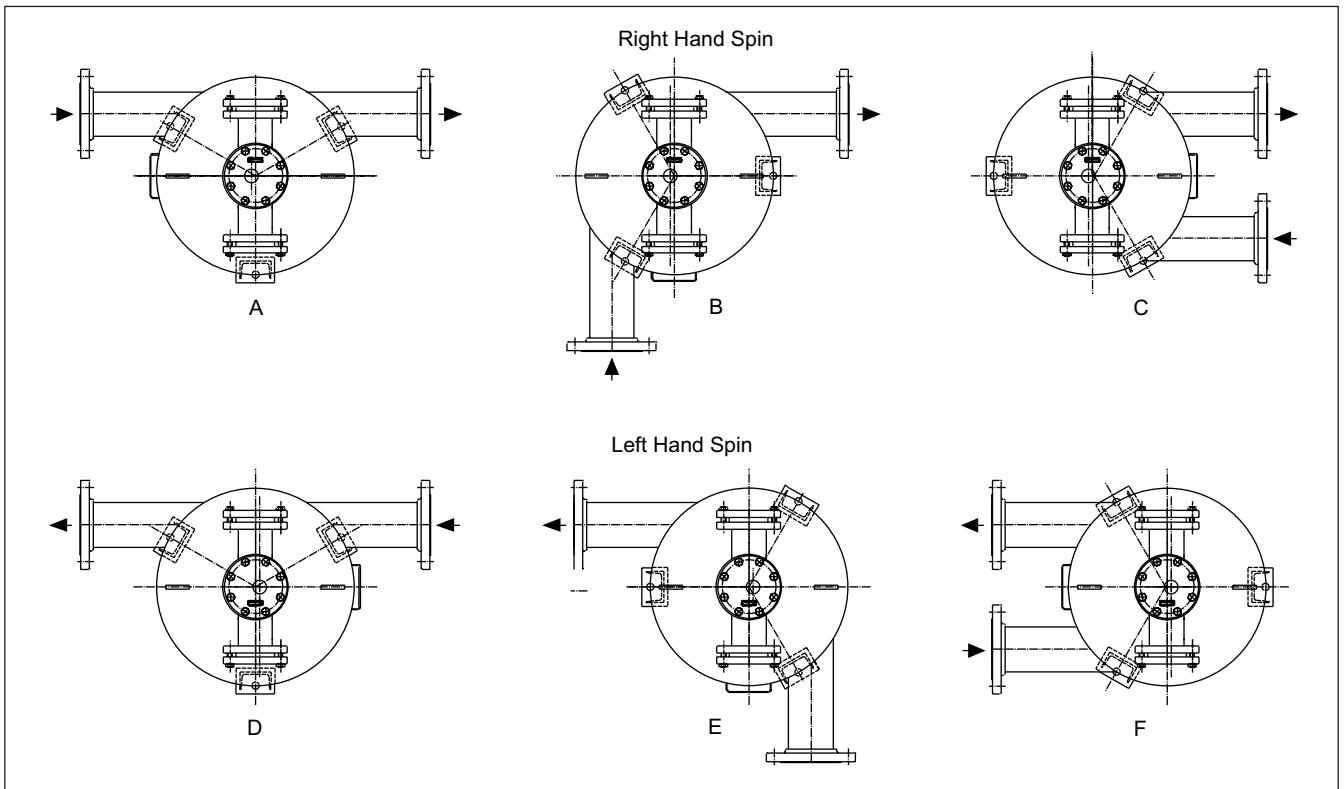
Figure 7 – Flange Arrangement and Flow Direction
