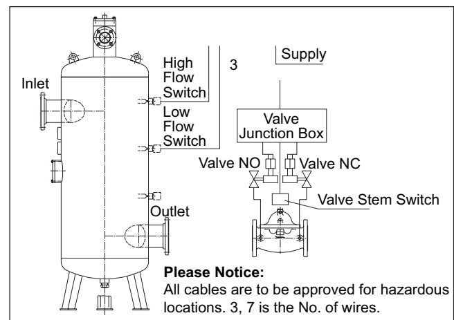
Figure 5 – Smith Meter Liquid Level Control Model 210 Digital Electro-Hydraulic Set-Stop Valve
