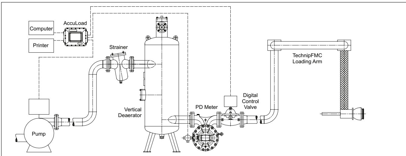
Figure 2 – Typical Installation for Loading Application
