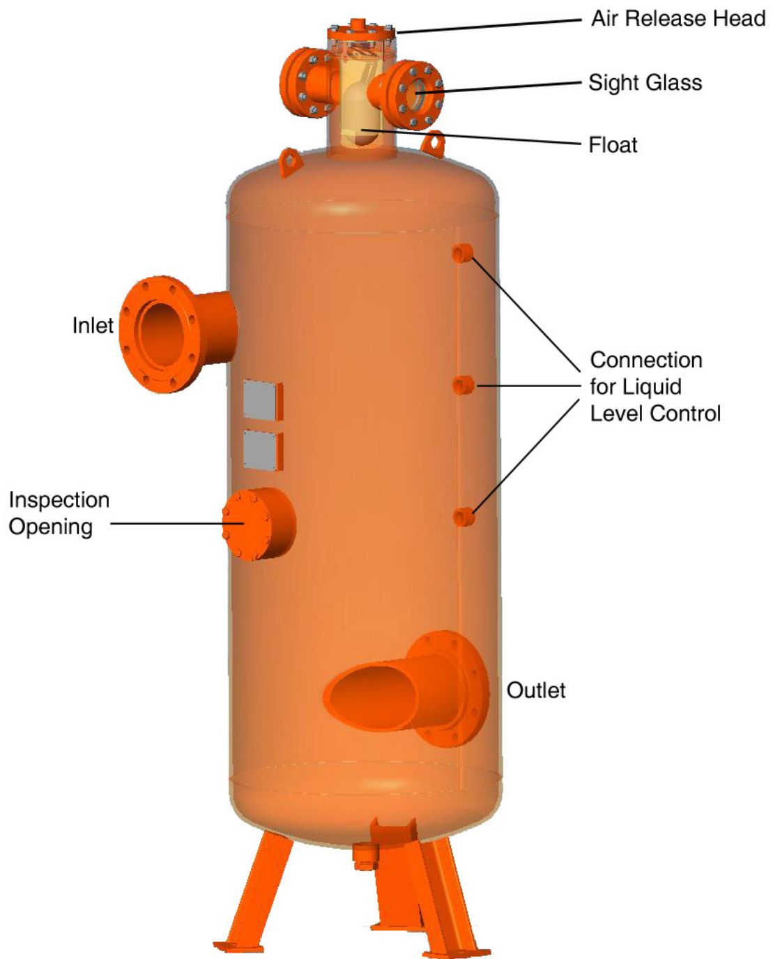
Figure 9 – VDR Deaerator Standard
