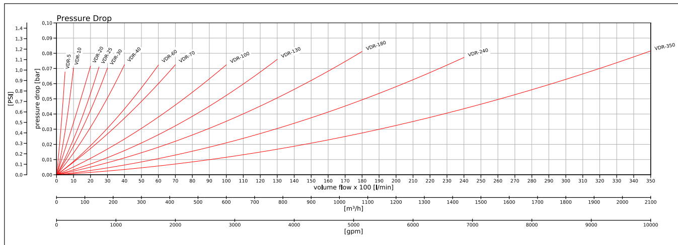
Figure 6 – Pressure Drop
