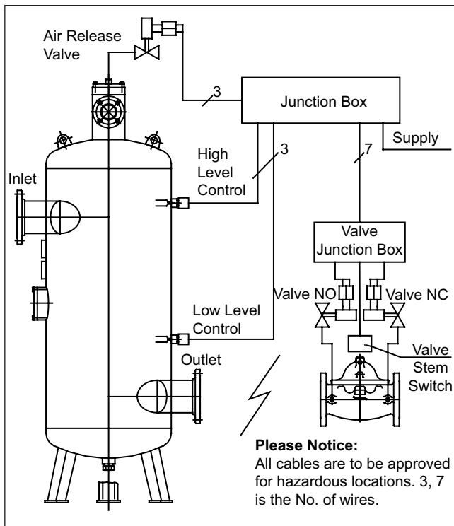
Figure 3 – Smith Meter Liquid Level Control Model 296 Set-Stop Valve
