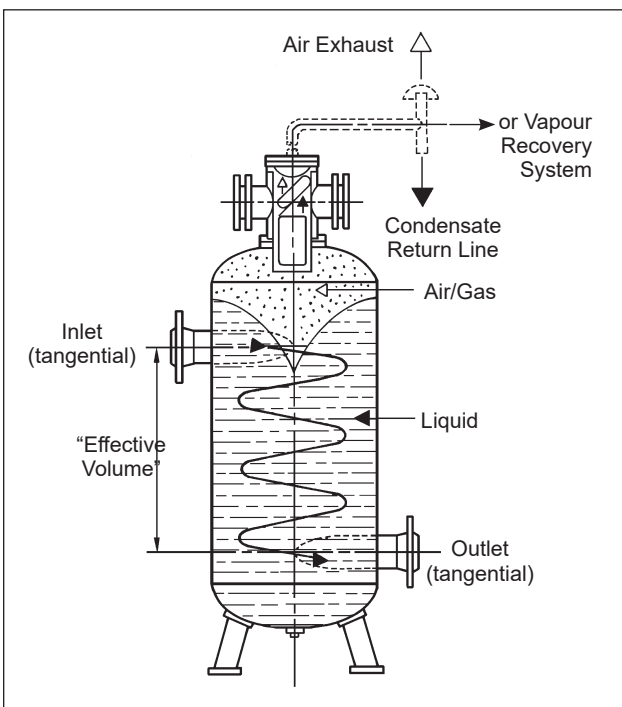
Figure 1 – VDR Deaerator
