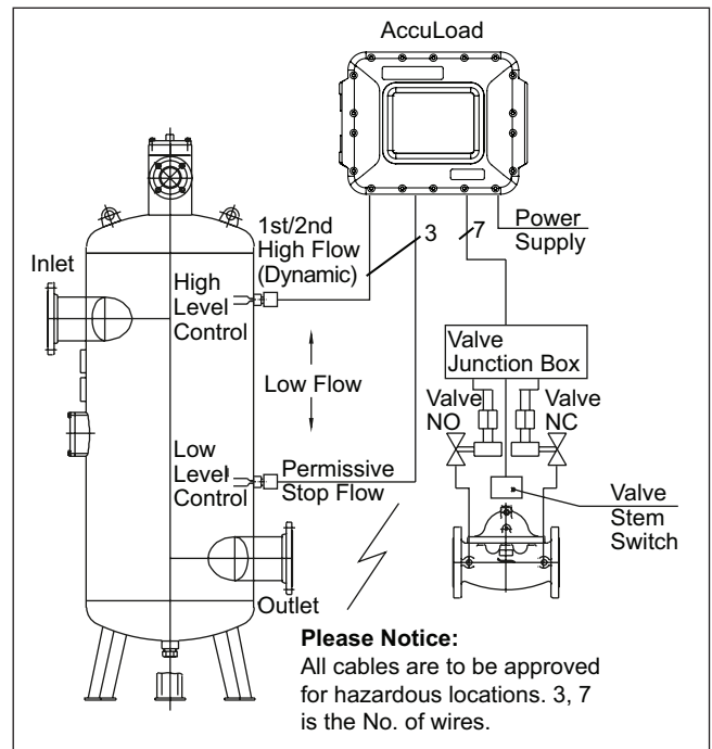
Figure 4 – Smith Meter Liquid Level Control Model 210 Digital Electro-Hydraulic Set-Stop Valve
