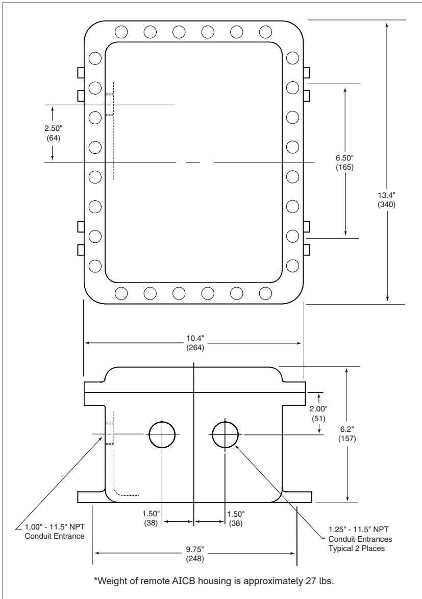
Figure 3 – Remote Housing (Optional AICB)
